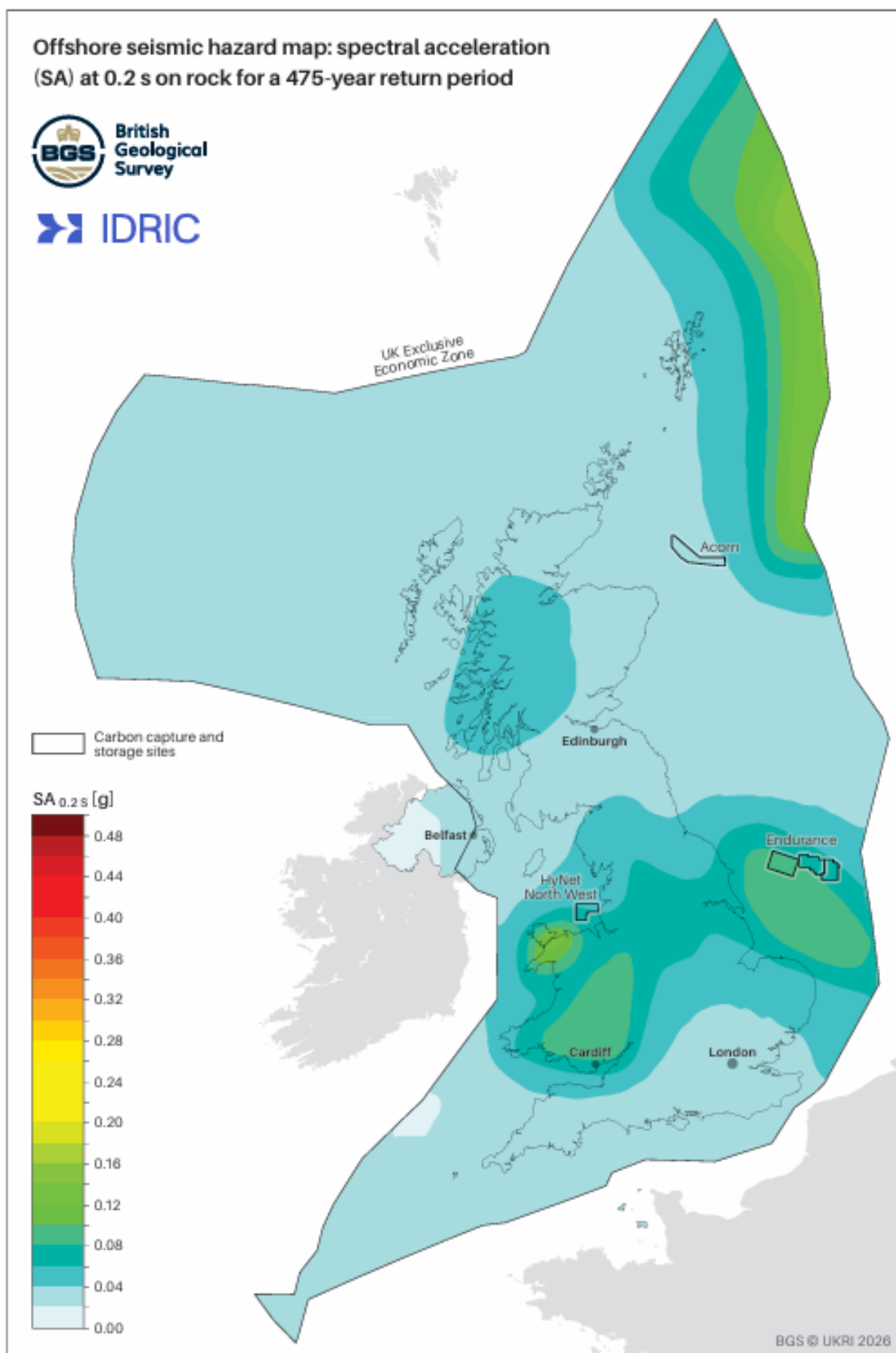
Figure 14 Hazard map for SA_{0.2s} for a 475-year return period. The large, black polygon describes the UK offshore EEZ. BGS © UKRI 2026. Contains OS data © Crown copyright and database right 2026.
