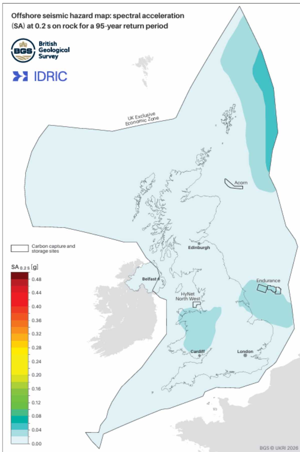
Figure 13 Hazard map for SA_{0.2\text{ s}} for a 95-year return period. The large, black polygon describes the UK offshore EEZ. BGS © UKRI 2026. Contains OS data © Crown copyright and database right 2026.
