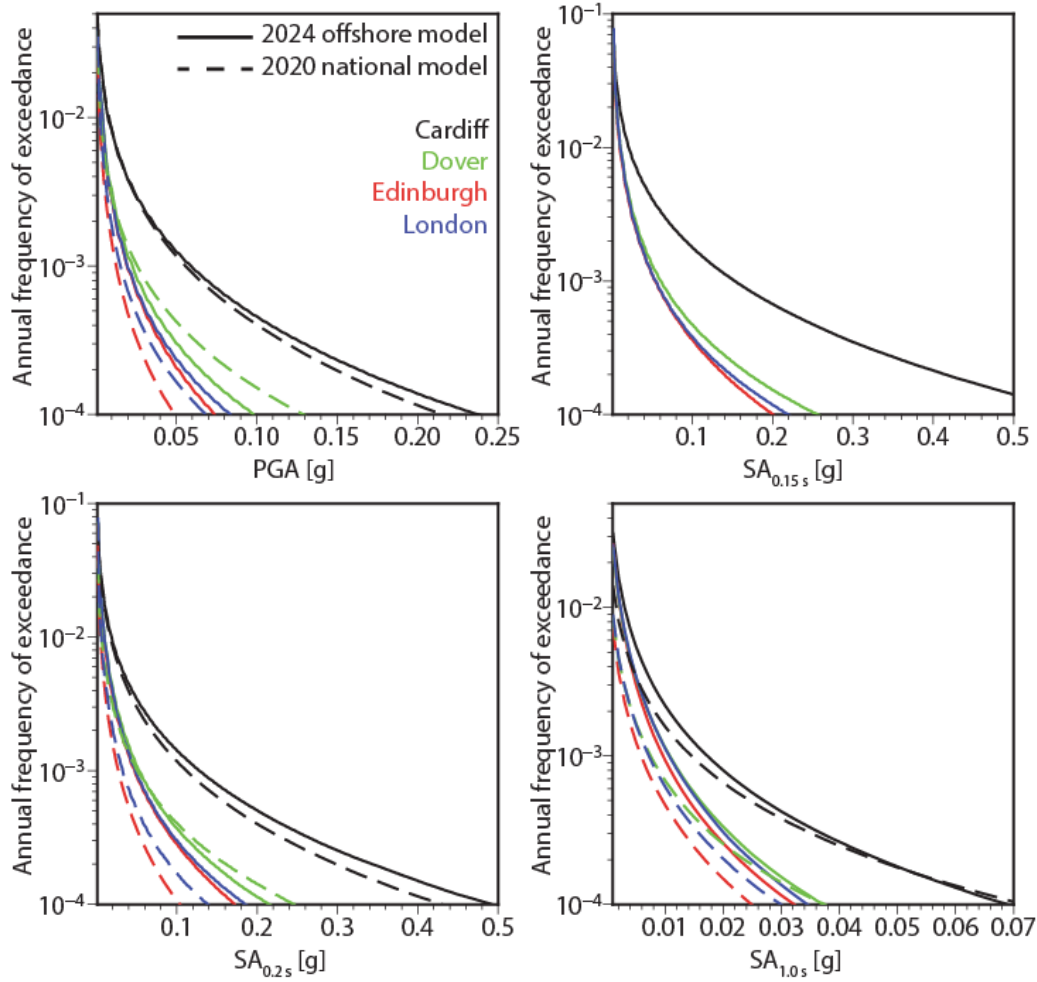
Figure 23 PGA, SA_{0.15s} , SA_{0.20s} , and SA_{1.00s} hazard curves for sites in Cardiff, Dover, Edinburgh, and London. Solid and dashed lines are the hazard curves computed using the 2024 offshore hazard model and the 2020 national hazard model, respectively.
