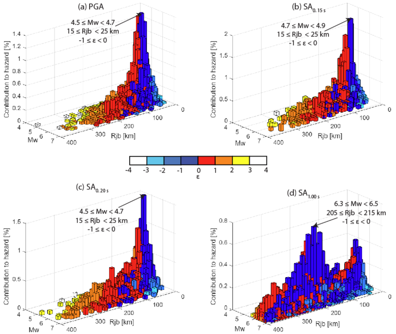
Figure 32 Disaggregation of the hazard for the London site and 2475-year return period by magnitude (Mw), Joyner-Boore distance (Rjb) and epsilon ( \epsilon ) for (a) PGA, (b) SA_{0.15s} , (c) SA_{0.20s} , and (d) SA_{1.00s} .
