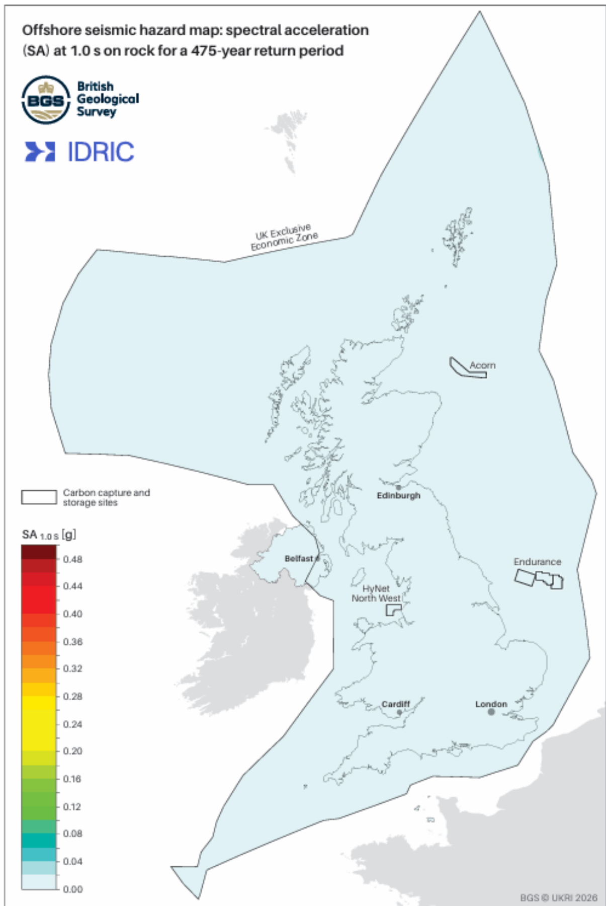
Figure 19 Hazard map for SA_{1.0s} for a 475-year return period. The large, black polygon describes the UK offshore EEZ. BGS © UKRI 2026. Contains OS data © Crown copyright and database right 2026.
