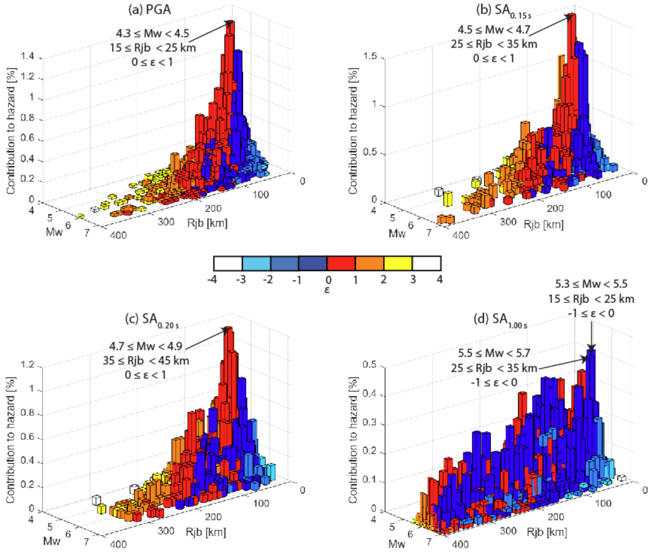
Figure 30 Disaggregation of the hazard for the Edinburgh site and 2475-year return period by magnitude (Mw), Joyner-Boore distance (Rjb) and epsilon ( \epsilon ) for (a) PGA, (b) SA_{0.15s} , (c) SA_{0.20s} , and (d) SA_{1.0s} .
