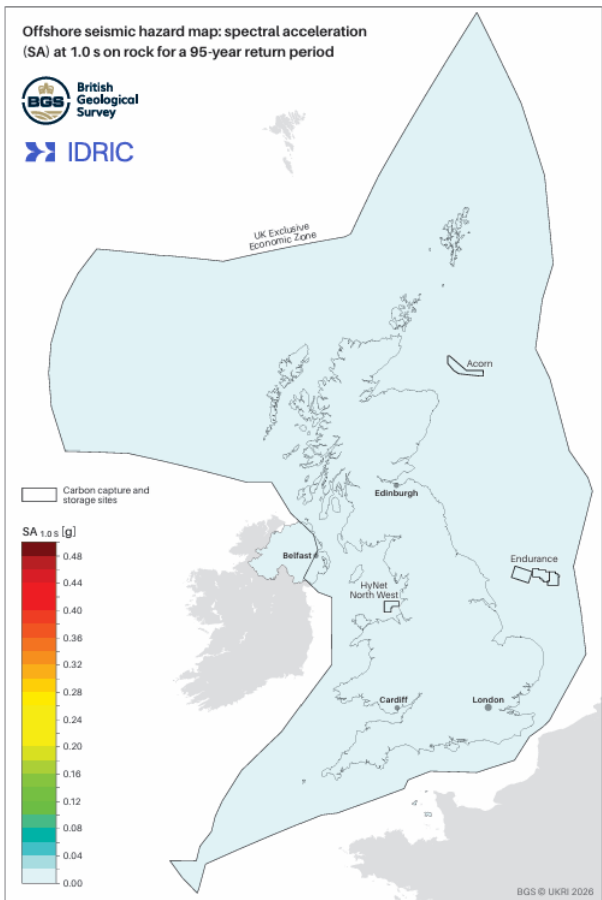
Figure 18 Hazard map for SA 1.00 s for a 95-year return period. The large, black polygon describes the UK offshore EEZ. BGS © UKRI 2026. Contains OS data © Crown copyright and database right 2026.
