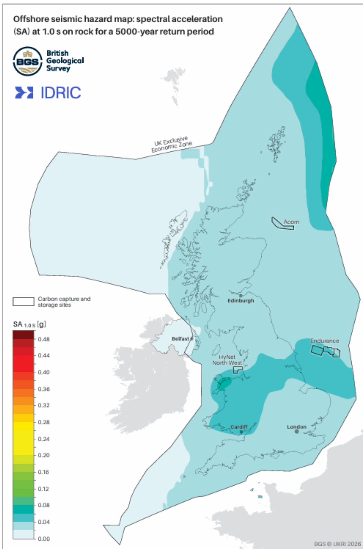
Figure 22 Hazard map for SA_{1.00\text{ s}} for a 5000-year return period. The large, black polygon describes the UK offshore EEZ. BGS © UKRI 2026. Contains OS data © Crown copyright and database right 2026.
