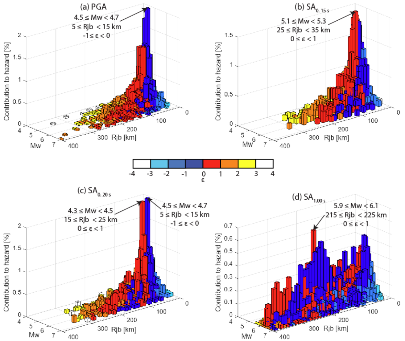
Figure 28 Disaggregation of the hazard for the Dover site and 2475-year return period by magnitude (Mw), Joyner-Boore distance (Rjb) and epsilon ( \epsilon ) for (a) PGA, (b) SA_{0.15 \text{ s}} , (c) SA_{0.20 \text{ s}} , and (d) SA_{1.00 \text{ s}} .
